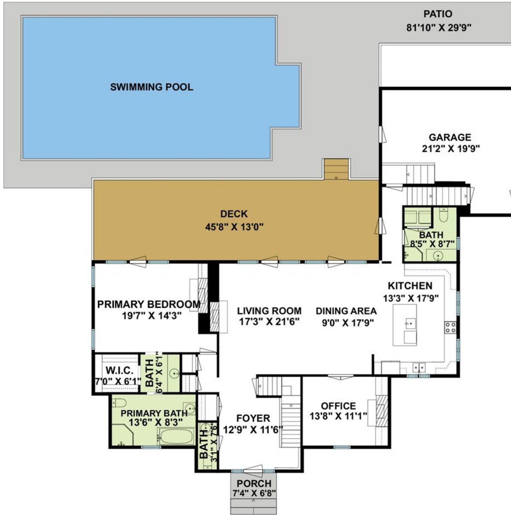
FIRST FLOOR
